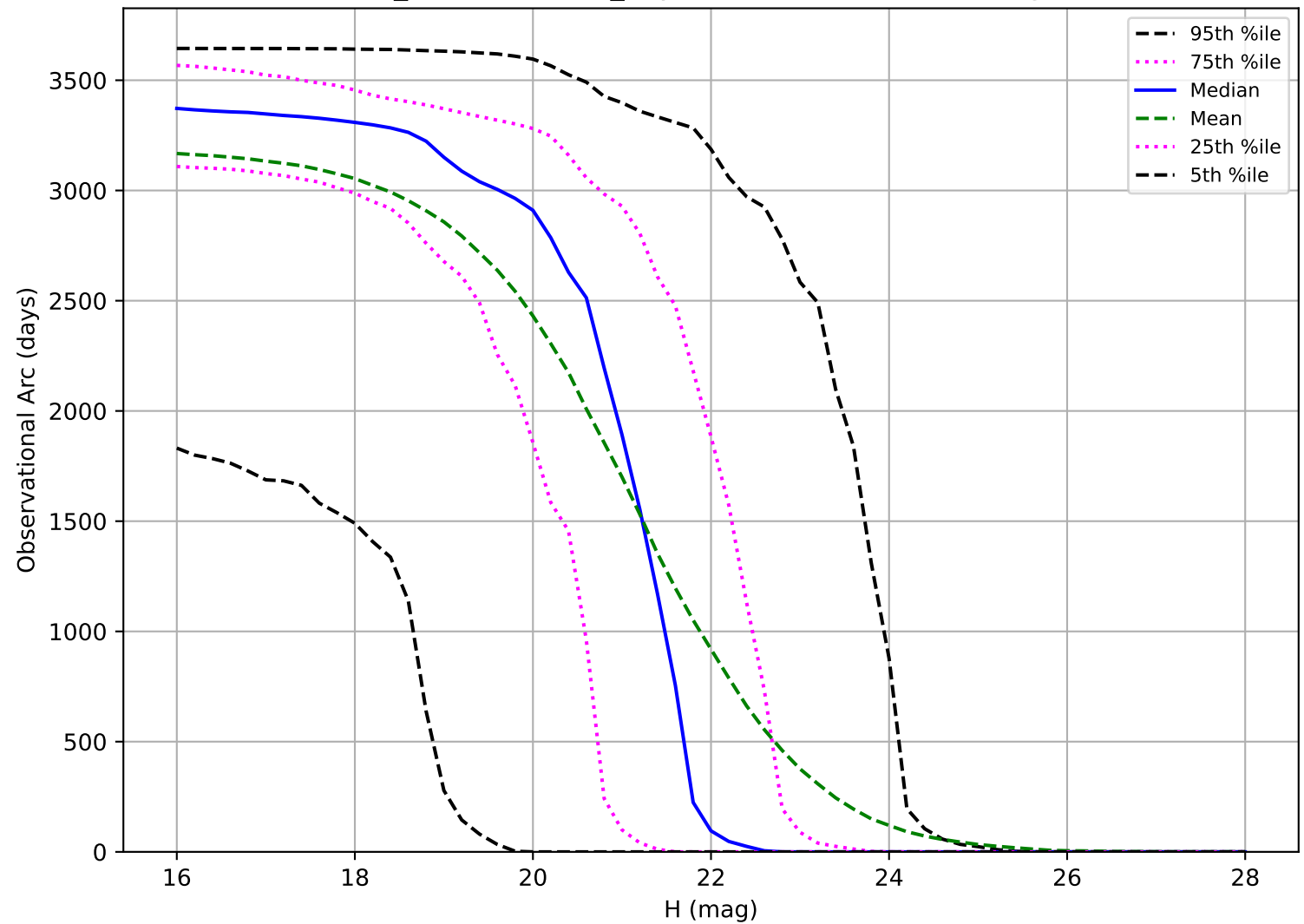
weather_cloudso36v3.4_10yrs: Observational Arc Length NEO
