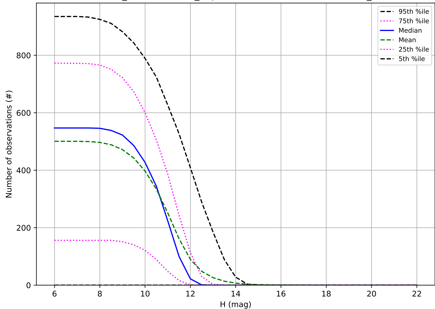
weather_cloudso36v3.4_10yrs: Number of observations OCC_r20
