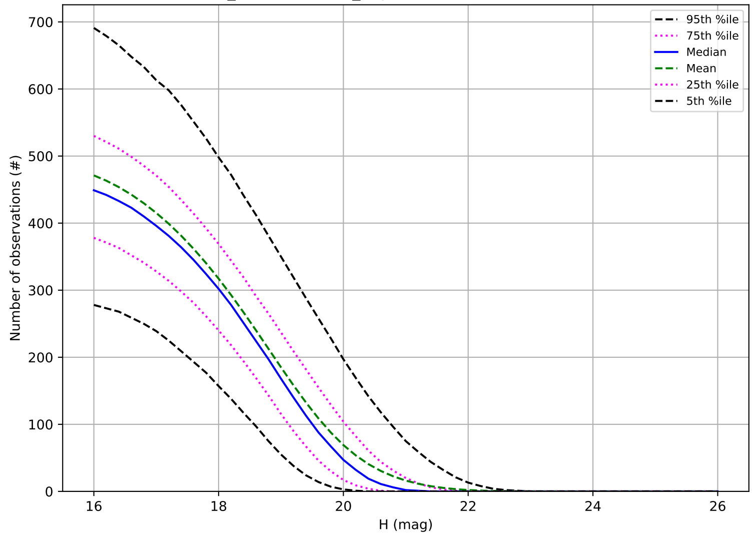
weather_cloudso36v3.4_10yrs: Number of observations MBA
