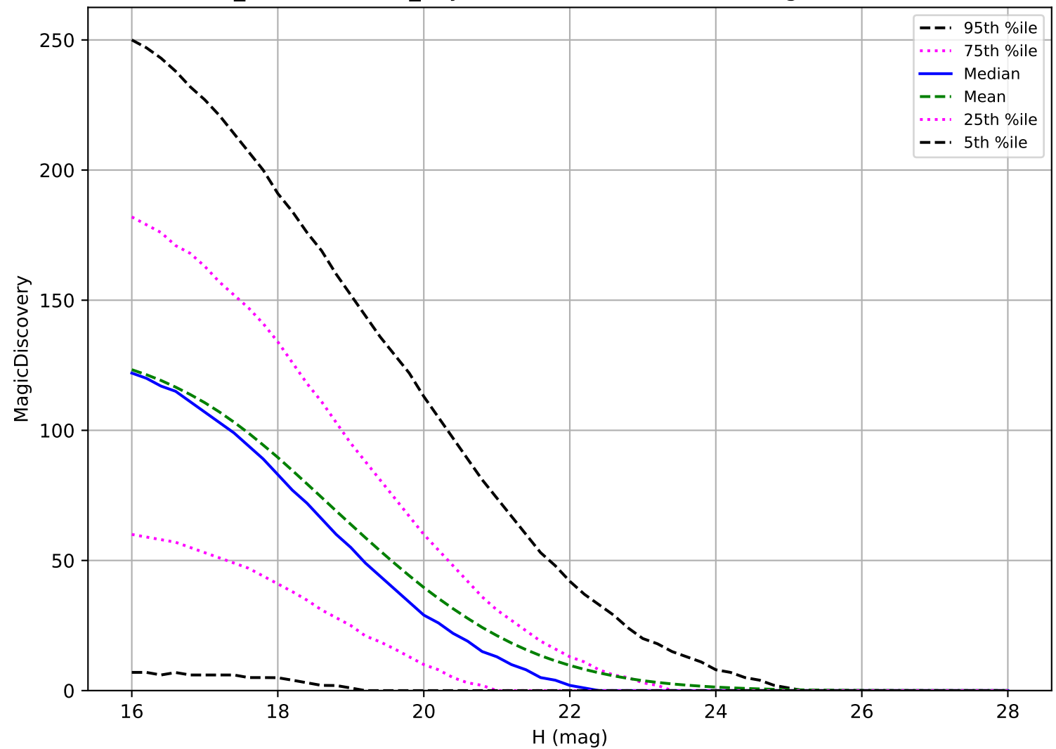
weather_cloudso36v3.4_10yrs: NEO 6 detections in 60 nights detection loss
