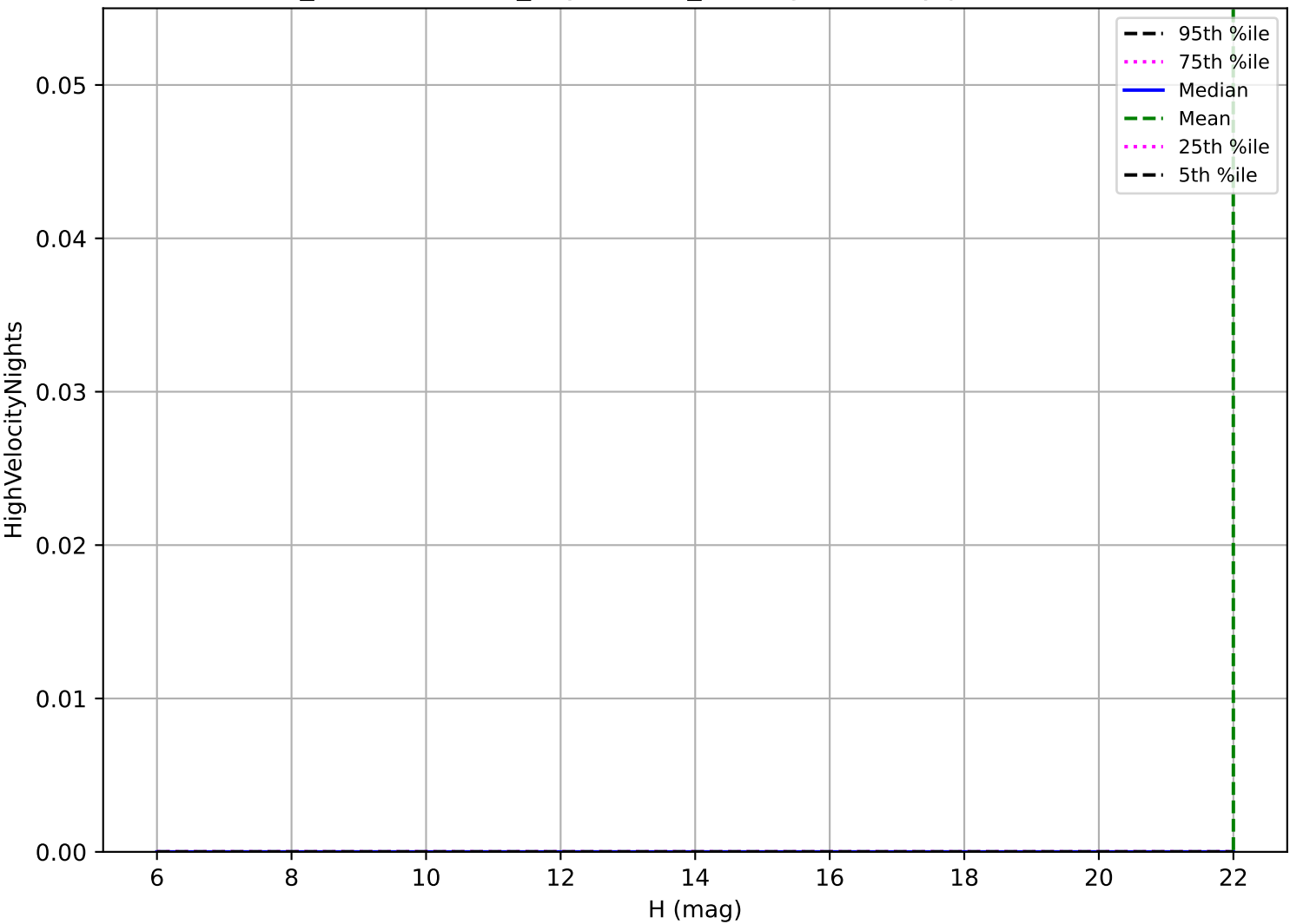
weather_cloudso36v3.4_10yrs: OCC_r20 High velocity pair detection loss
