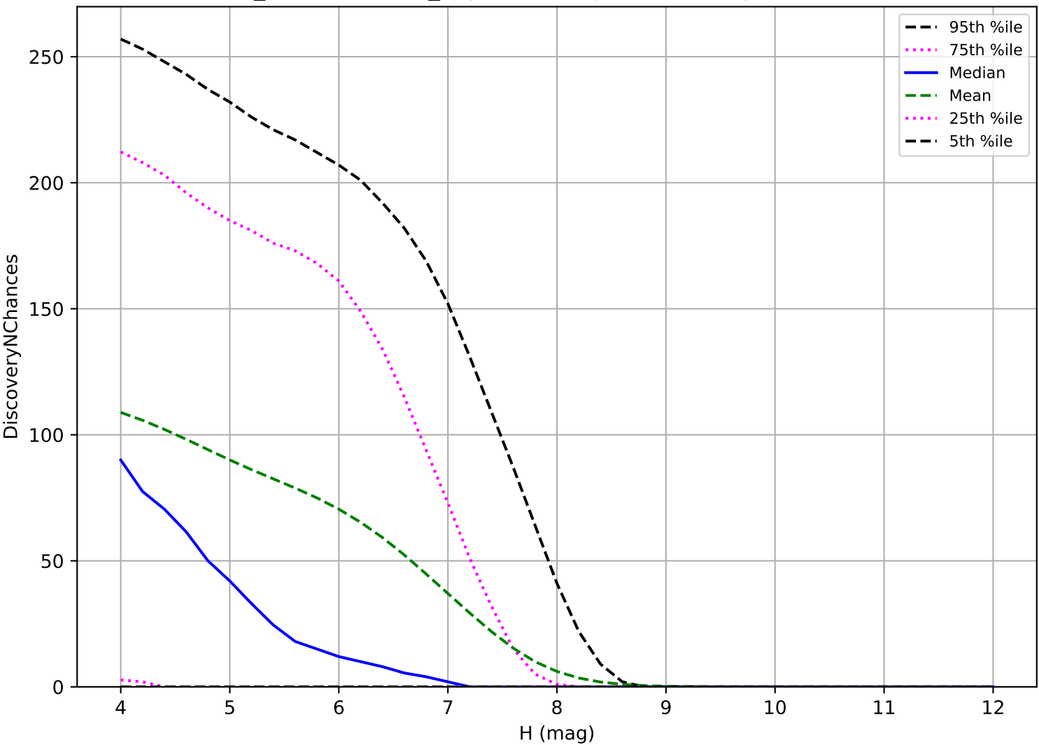
weather_cloudso36v3.4_10yrs: TNO 3 pairs in 15 nights detection loss
