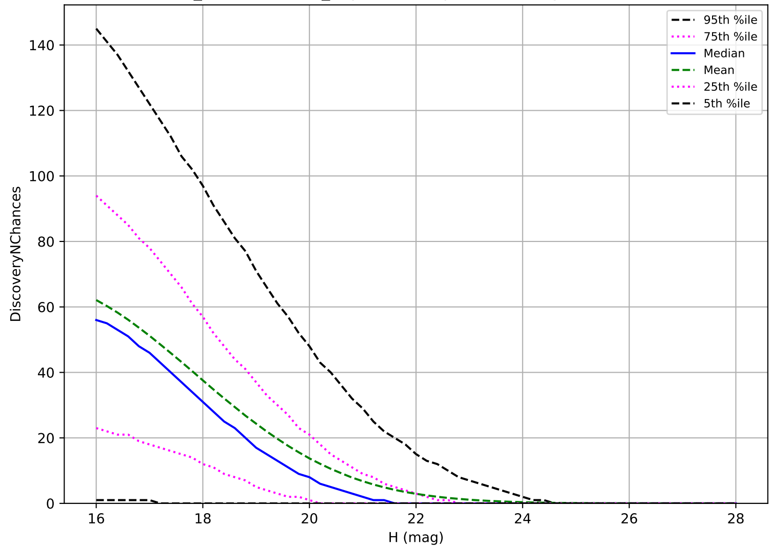
weather_cloudso36v3.4_10yrs: NEO 3 pairs in 15 nights detection loss
