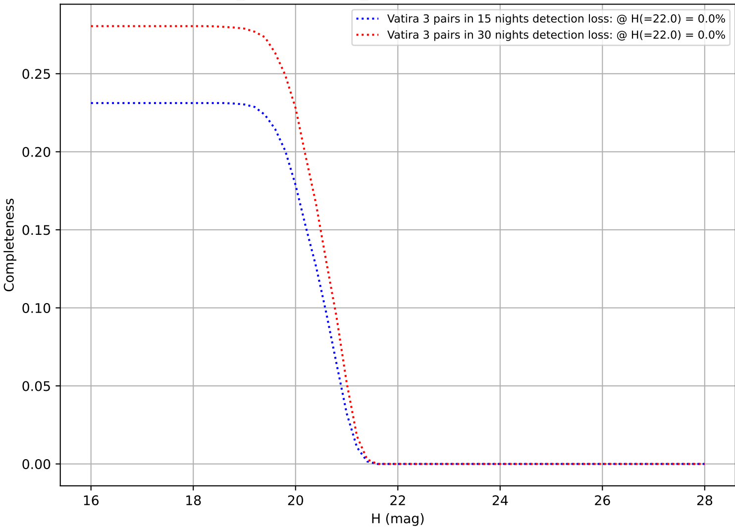
weather_cloudso36v3.4_10yrs: DifferentialCompleteness
