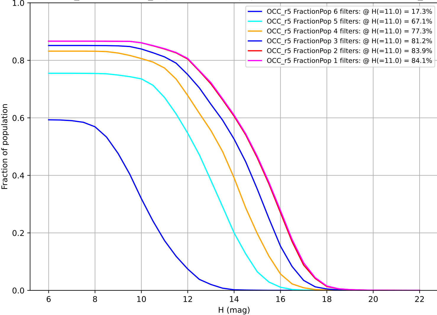
weather_cloudso36v3.4_10yrs: Fraction of population with colors in X filters OCC_r5
