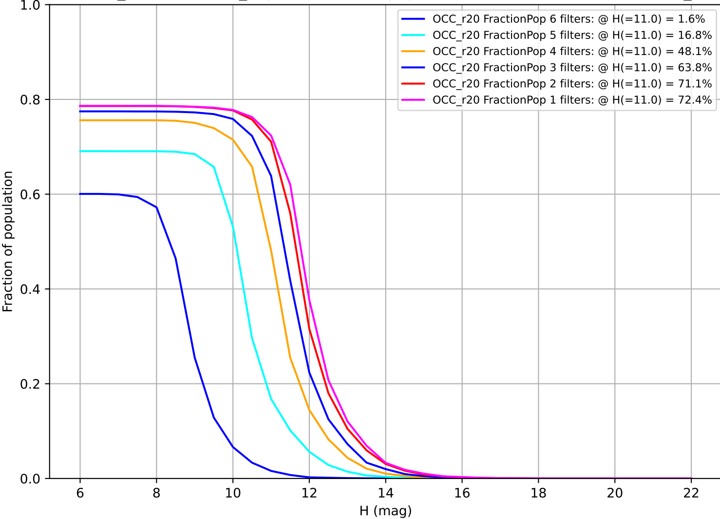
weather_cloudso36v3.4_10yrs: Fraction of population with colors in X filters OCC_r20
