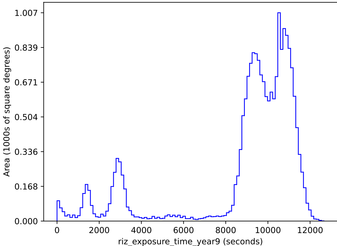
weather_cloudso36v3.4_10yrs gri band non-DD: riz_exposure_time_year9
