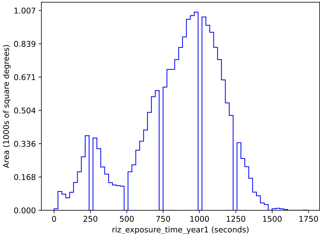
weather_cloudso36v3.4_10yrs gri band non-DD: riz_exposure_time_year1
