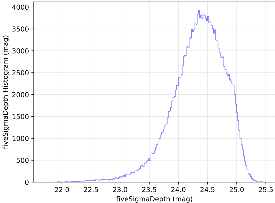
weather_cloudso36v3.4_10yrs g: fiveSigmaDepth Histogram
