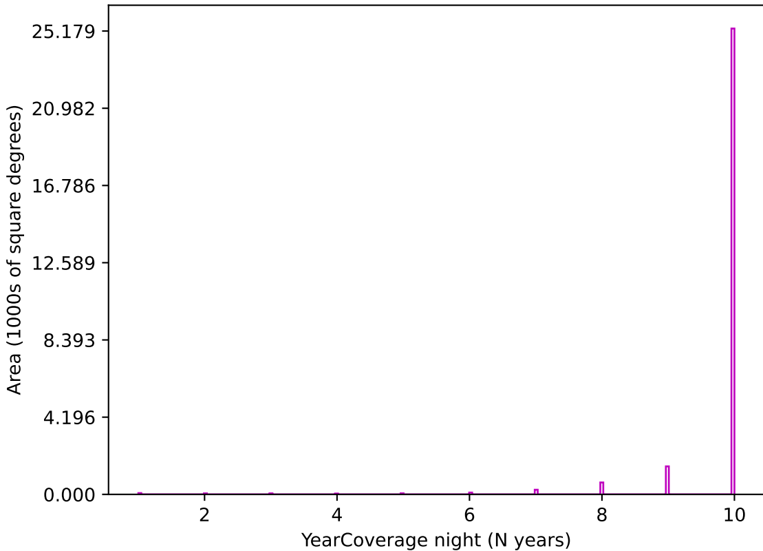
weather_cloudso36v3.4_10yrs z band: YearCoverage night
