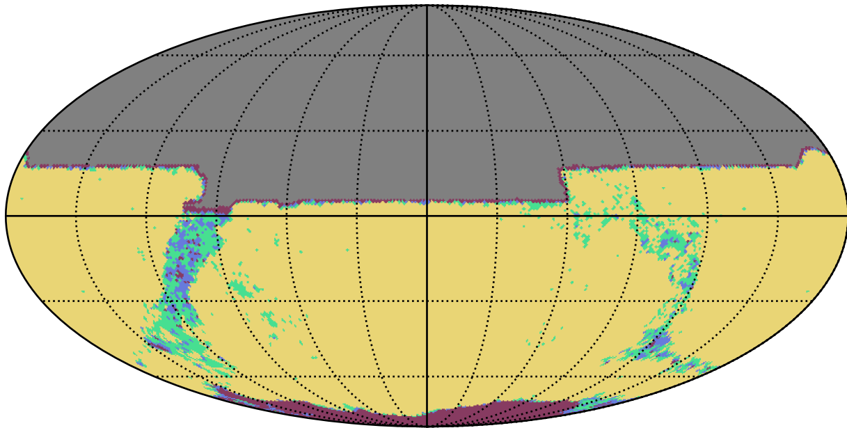
weather_cloudso36v3.4_10yrs y band: YearCoverage night
