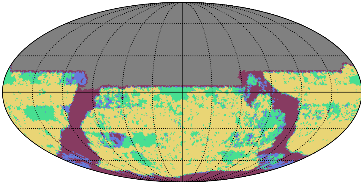
weather_cloudso36v3.4_10yrs u band: YearCoverage night
