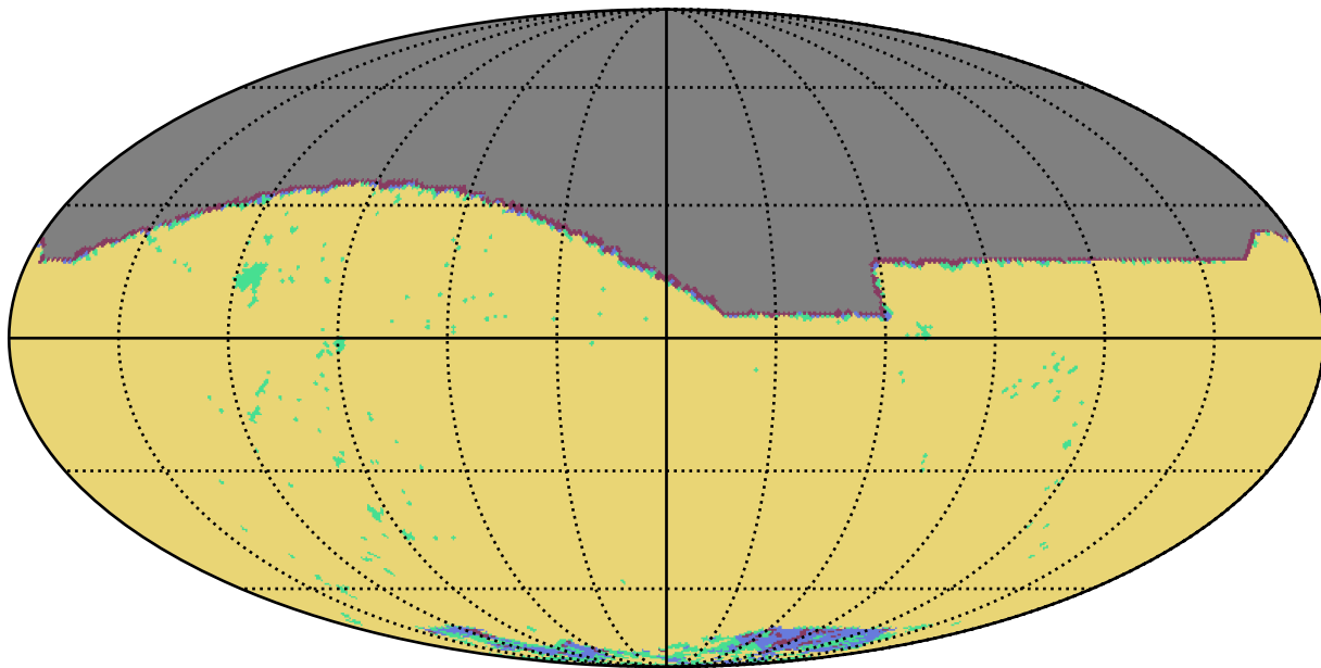
weather_cloudso36v3.4_10yrs i band: YearCoverage night
