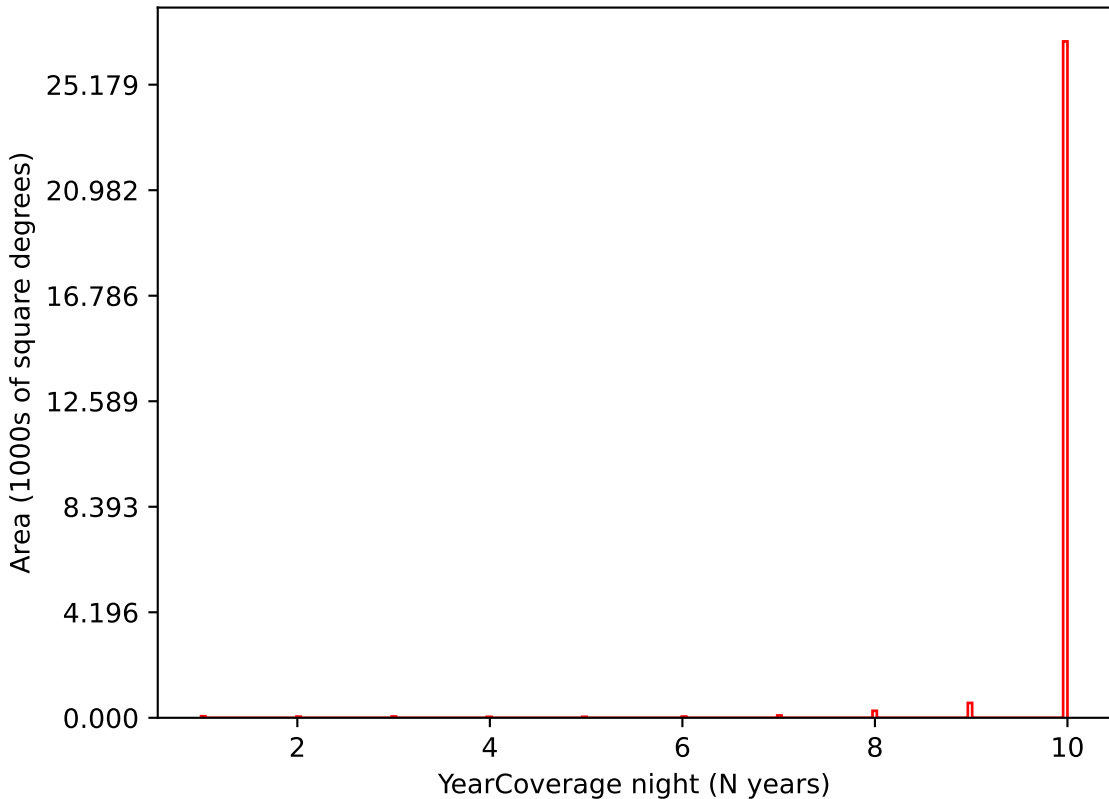
weather_cloudso36v3.4_10yrs i band: YearCoverage night
