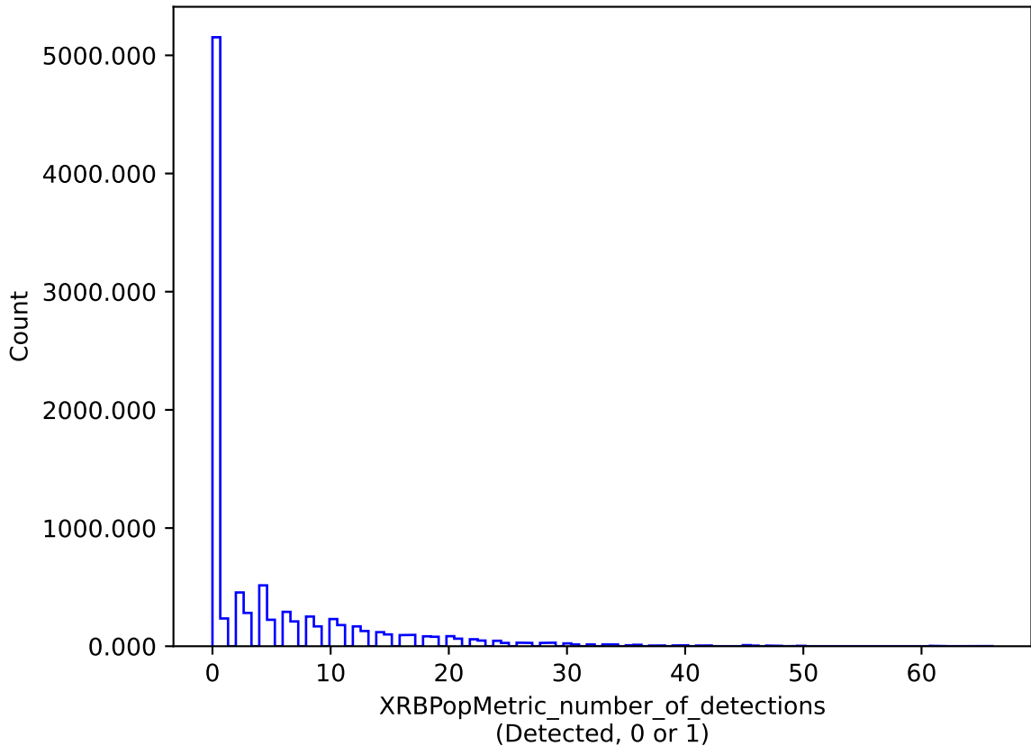
weather_cloudso36v3.4_10yrs : XRBPoMetric_number_of_detections
