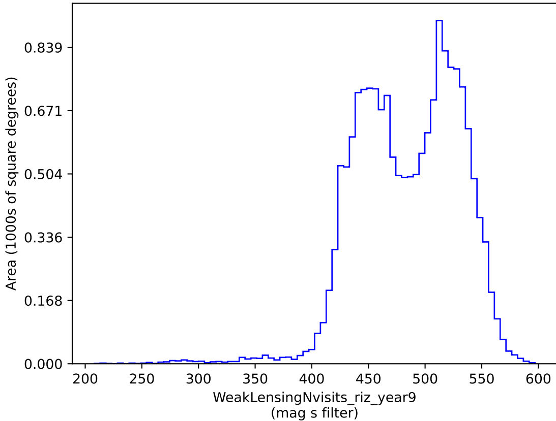
weather_cloudso36v3.4_10yrs gri band non-DD: WeakLensingNvisits_riz_year9
