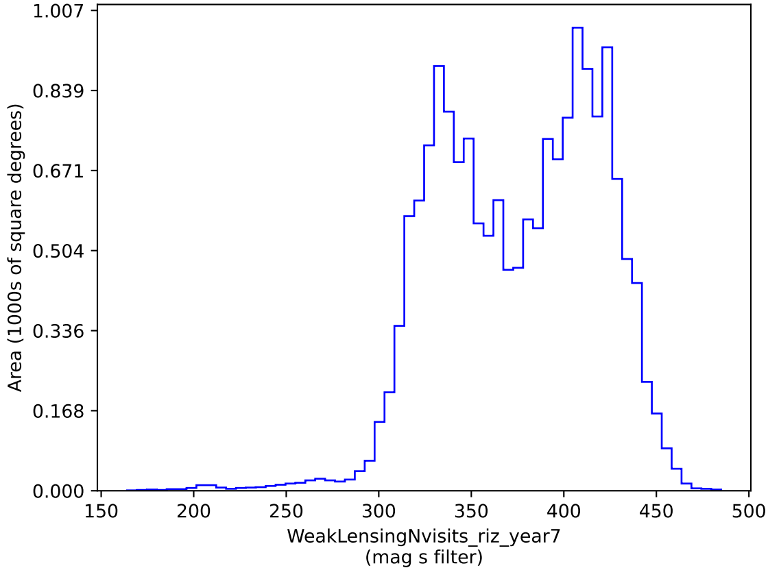
weather_cloudso36v3.4_10yrs gri band non-DD: WeakLensingNvisits_riz_year7
