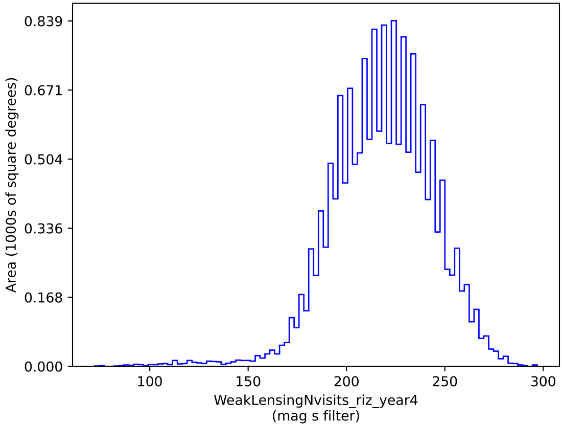
weather_cloudso36v3.4_10yrs gri band non-DD: WeakLensingNvisits_riz_year4
