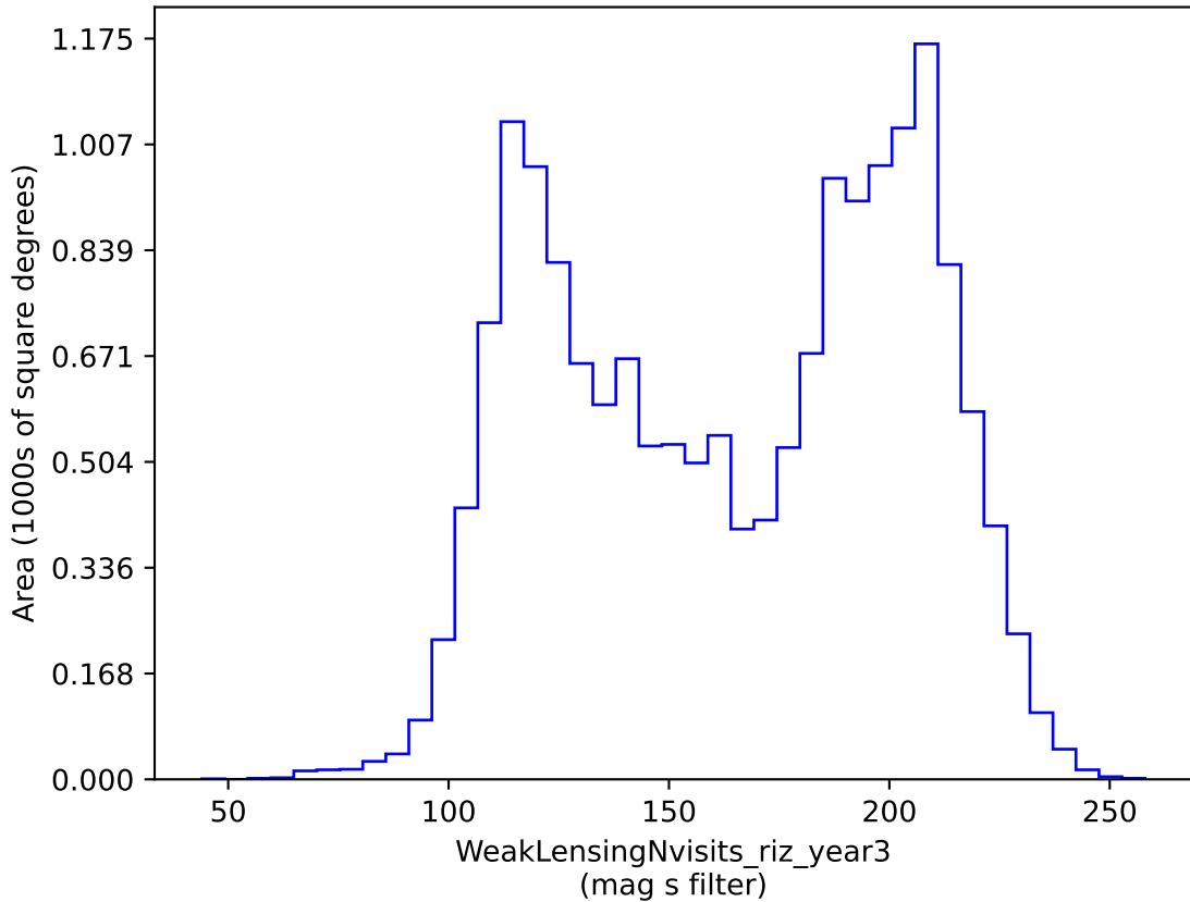
weather_cloudso36v3.4_10yrs gri band non-DD: WeakLensingNvisits_riz_year3
