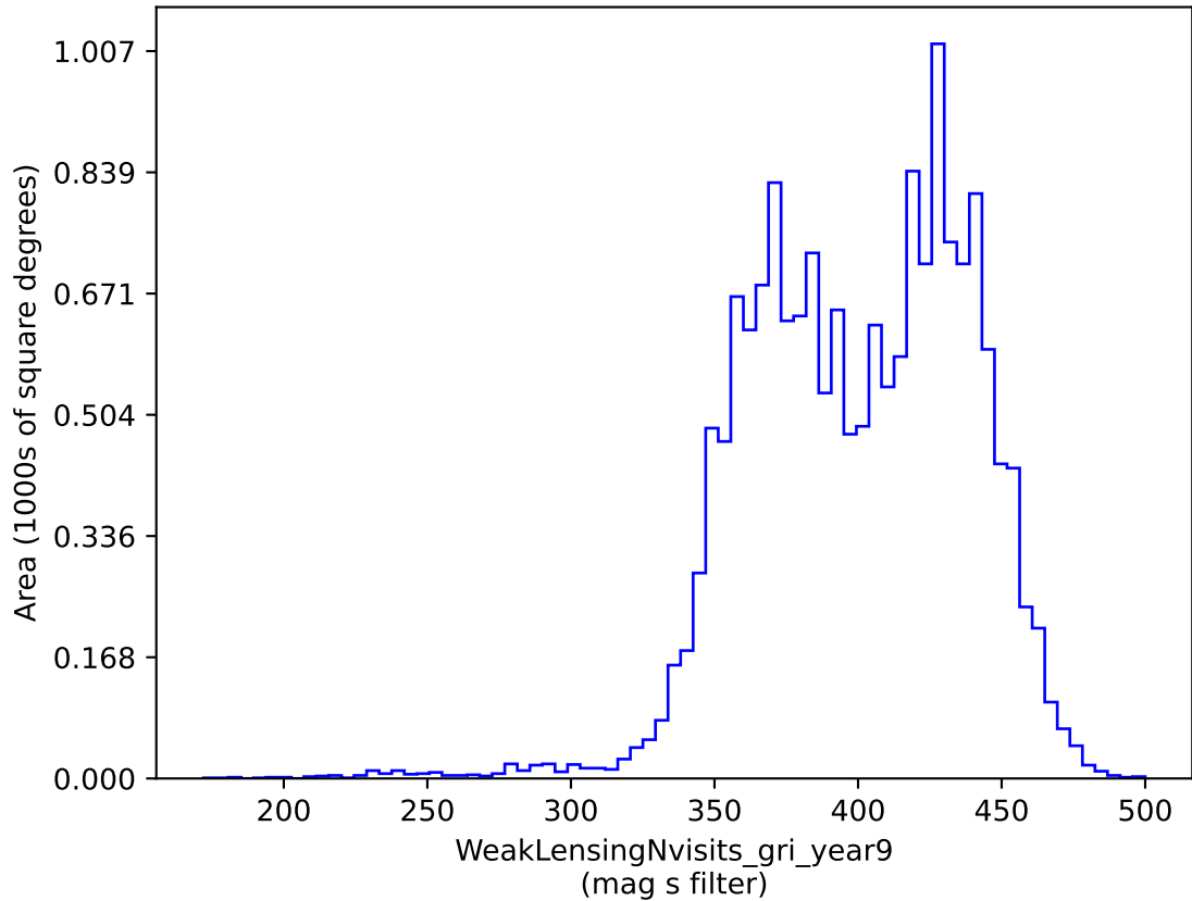
weather_cloudso36v3.4_10yrs gri band non-DD: WeakLensingNvisits_gri_year9
