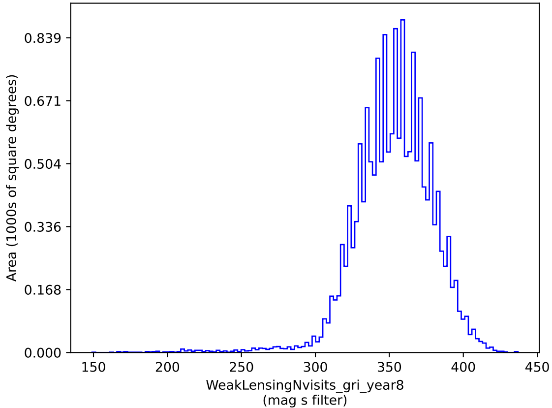
weather_cloudso36v3.4_10yrs gri band non-DD: WeakLensingNvisits_gri_year8
