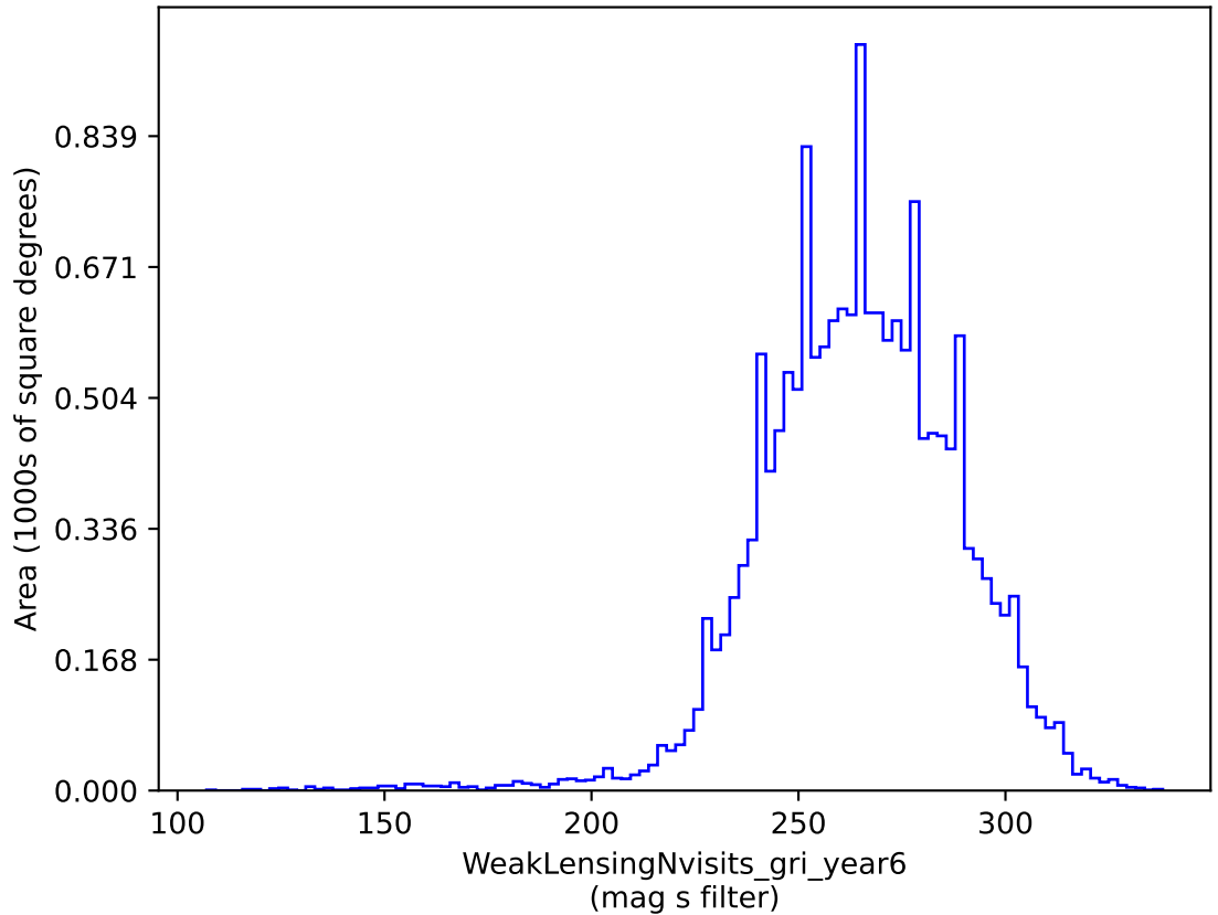
weather_cloudso36v3.4_10yrs gri band non-DD: WeakLensingNvisits_gri_year6
