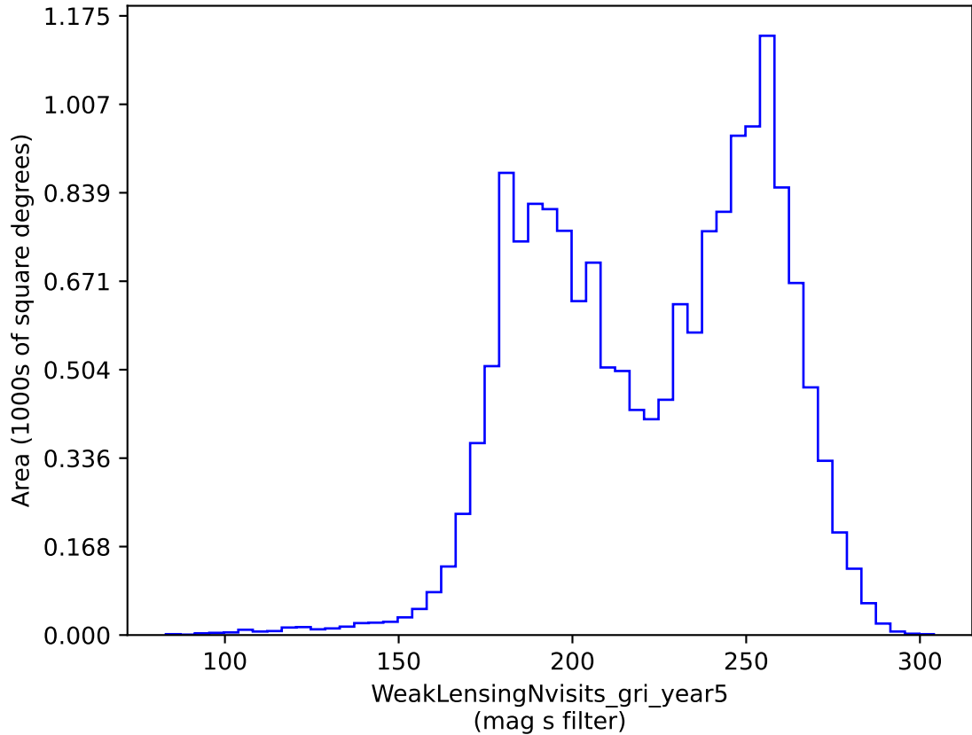
weather_cloudso36v3.4_10yrs gri band non-DD: WeakLensingNvisits_gri_year5
