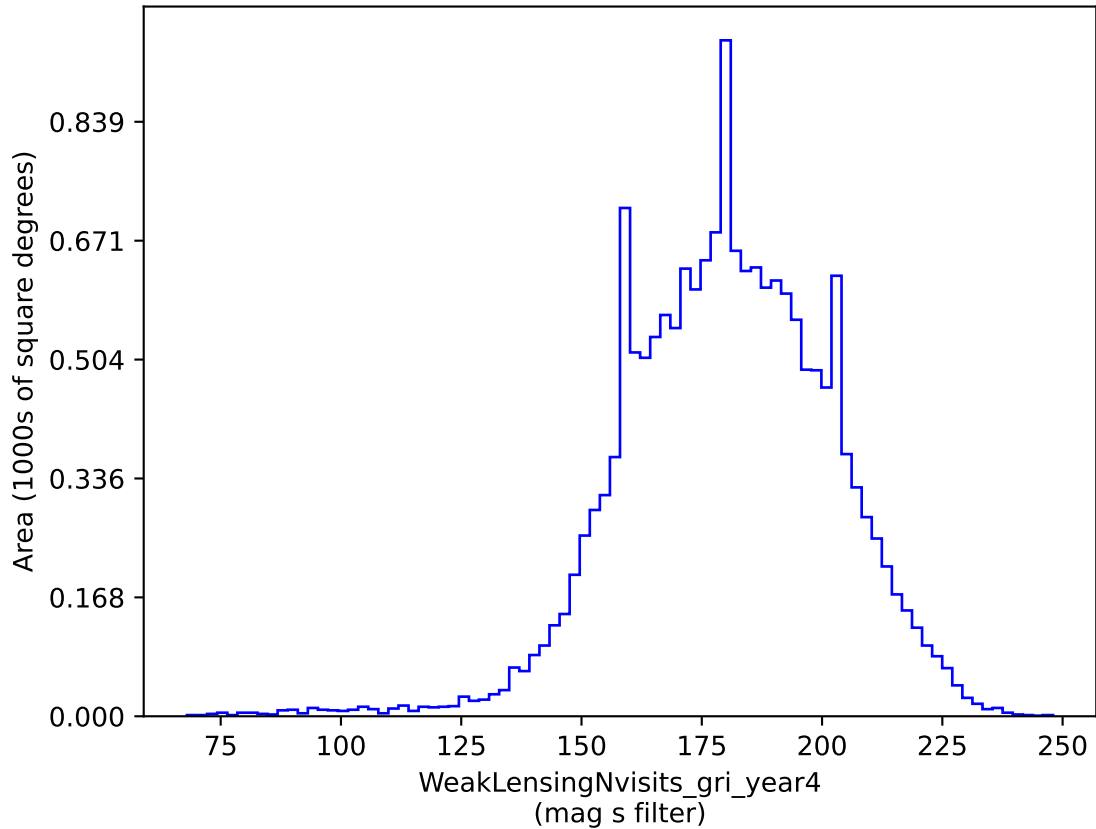
weather_cloudso36v3.4_10yrs gri band non-DD: WeakLensingNvisits_gri_year4
