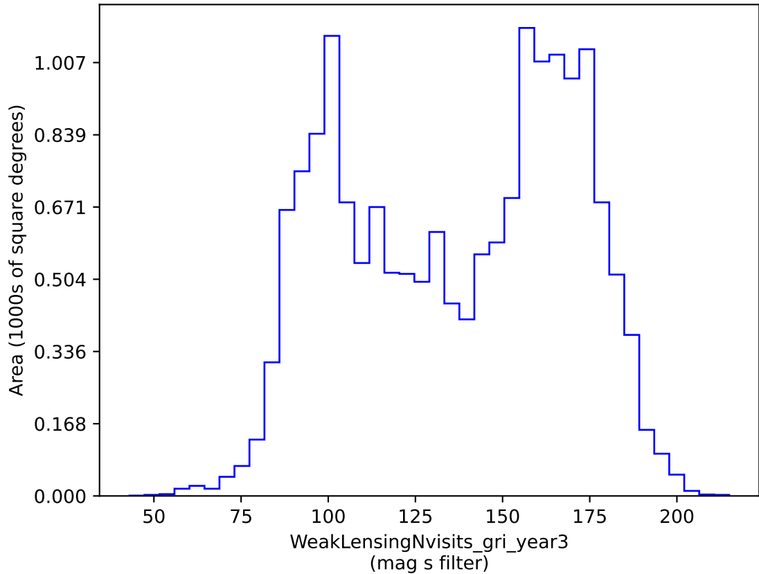
weather_cloudso36v3.4_10yrs gri band non-DD: WeakLensingNvisits_gri_year3
