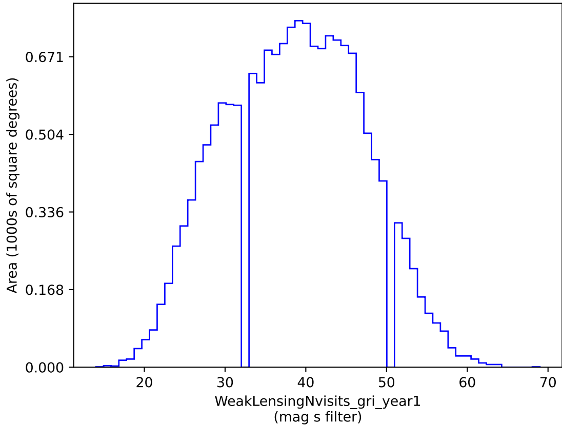
weather_cloudso36v3.4_10yrs gri band non-DD: WeakLensingNvisits_gri_year1
