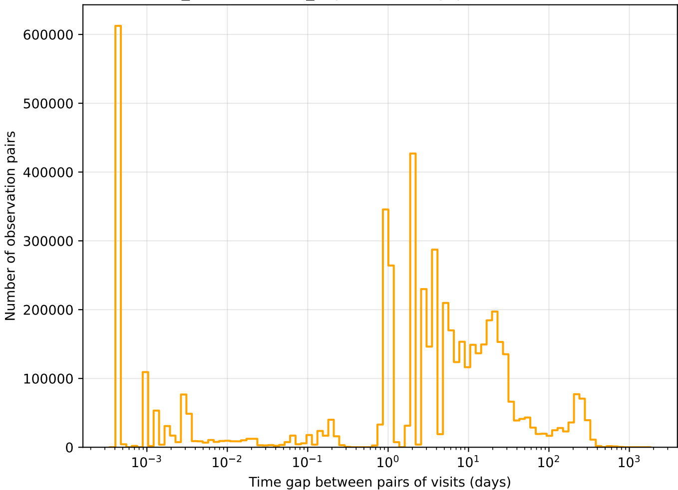
weather_cloudso36v3.4_10yrs r band: Tgaps observationStartMJD
