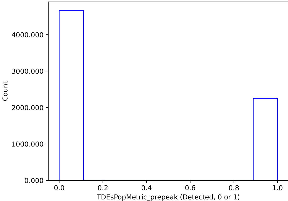
weather_cloudso36v3.4_10yrs : TDEsPopMetric_prepeak
