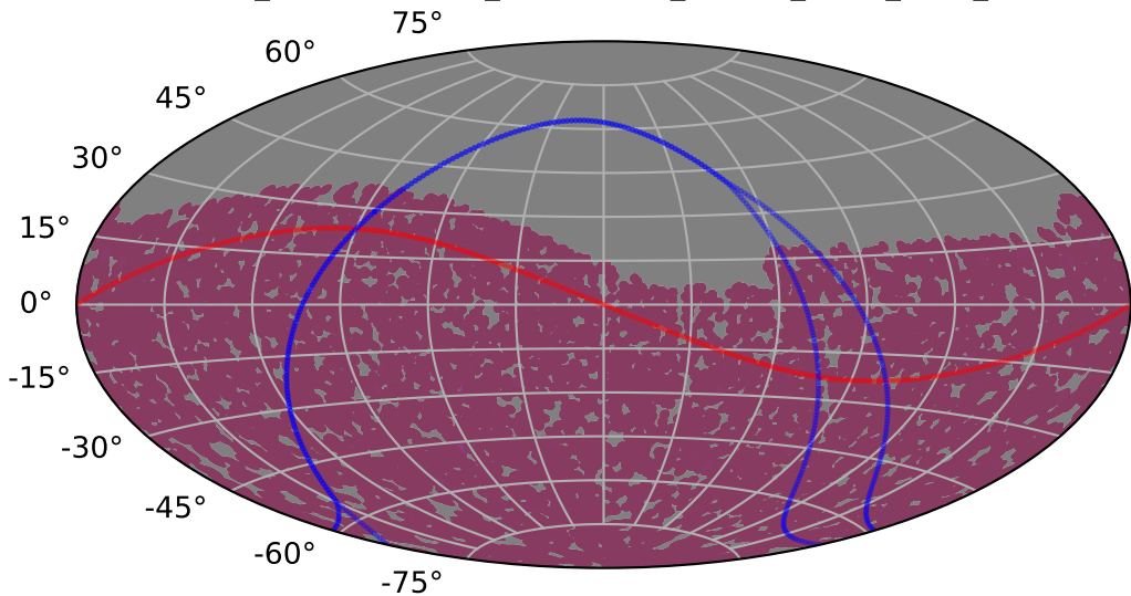
weather_cloudso36v3.4_10yrs : TDE_Quality_some_color_pnum
