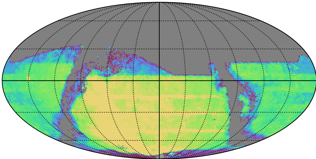
weather_cloudso36v3.4_10yrs : TDC_season
