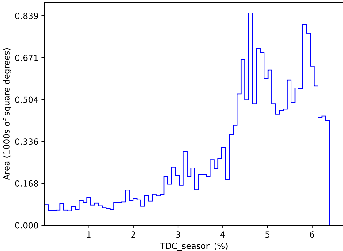
weather_cloudso36v3.4_10yrs : TDC_season
