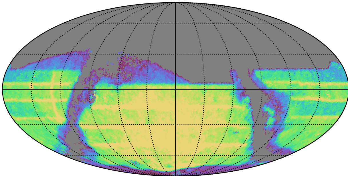
weather_cloudso36v3.4_10yrs : TDC_rate
