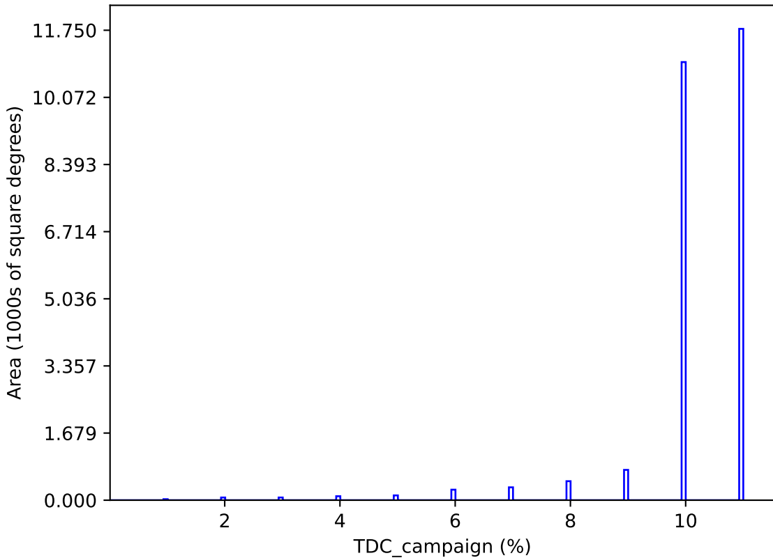
weather_cloudso36v3.4_10yrs : TDC_campaign
