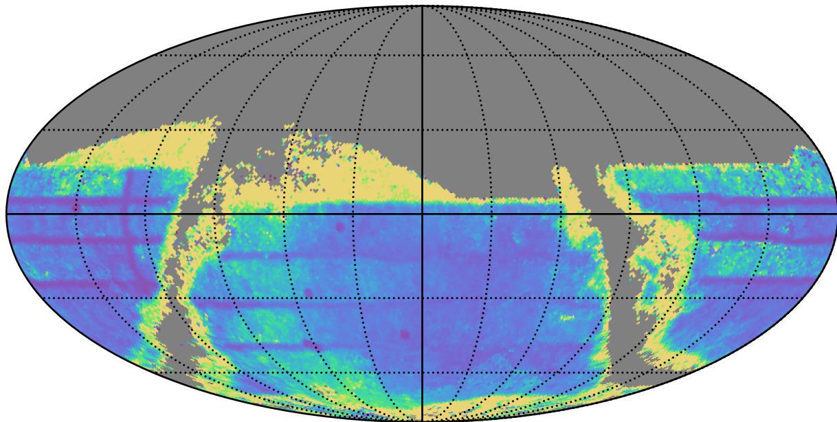
weather_cloudso36v3.4_10yrs : TDC_cadence
