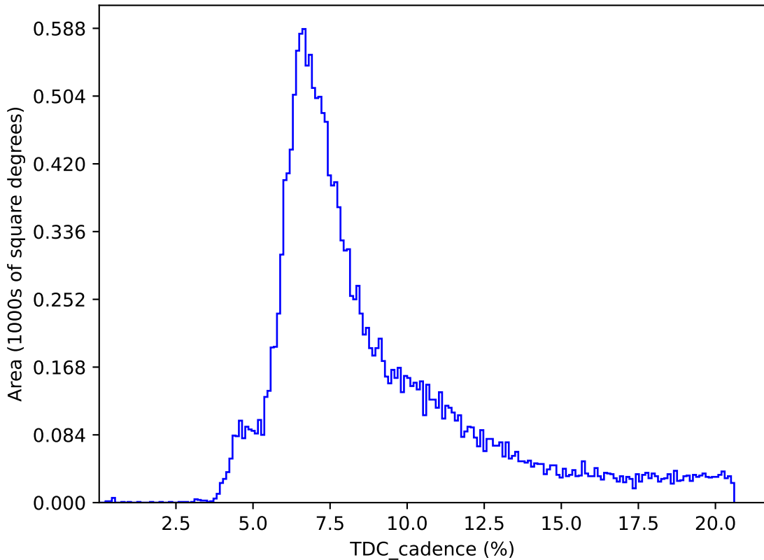
weather_cloudso36v3.4_10yrs : TDC_cadence
