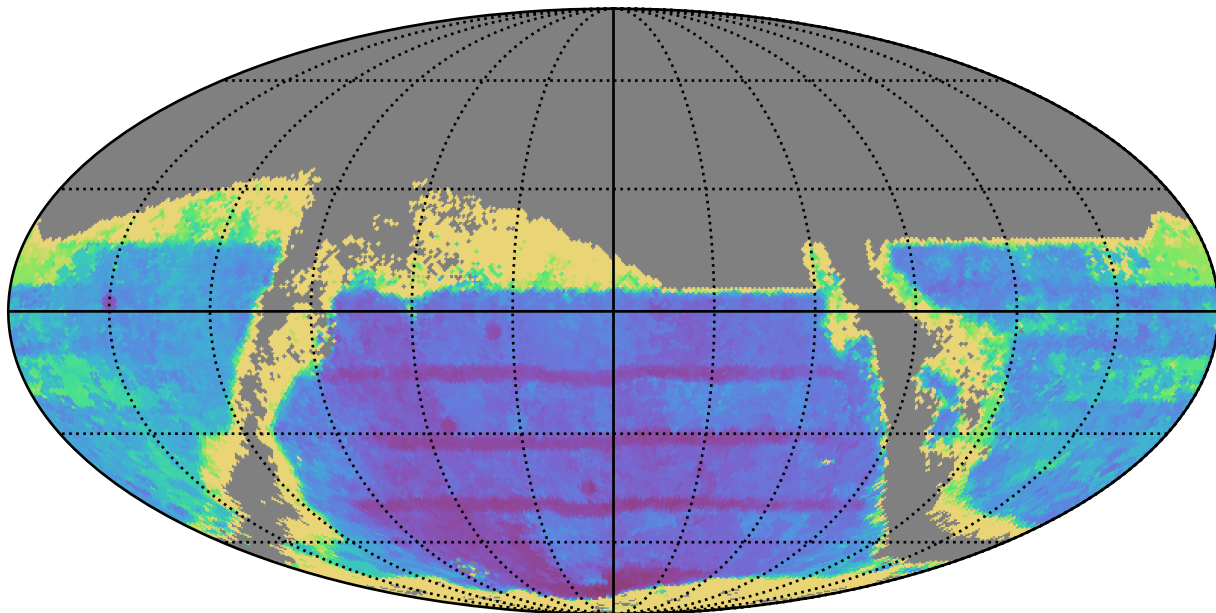
weather_cloudso36v3.4_10yrs : TDC_accuracy
