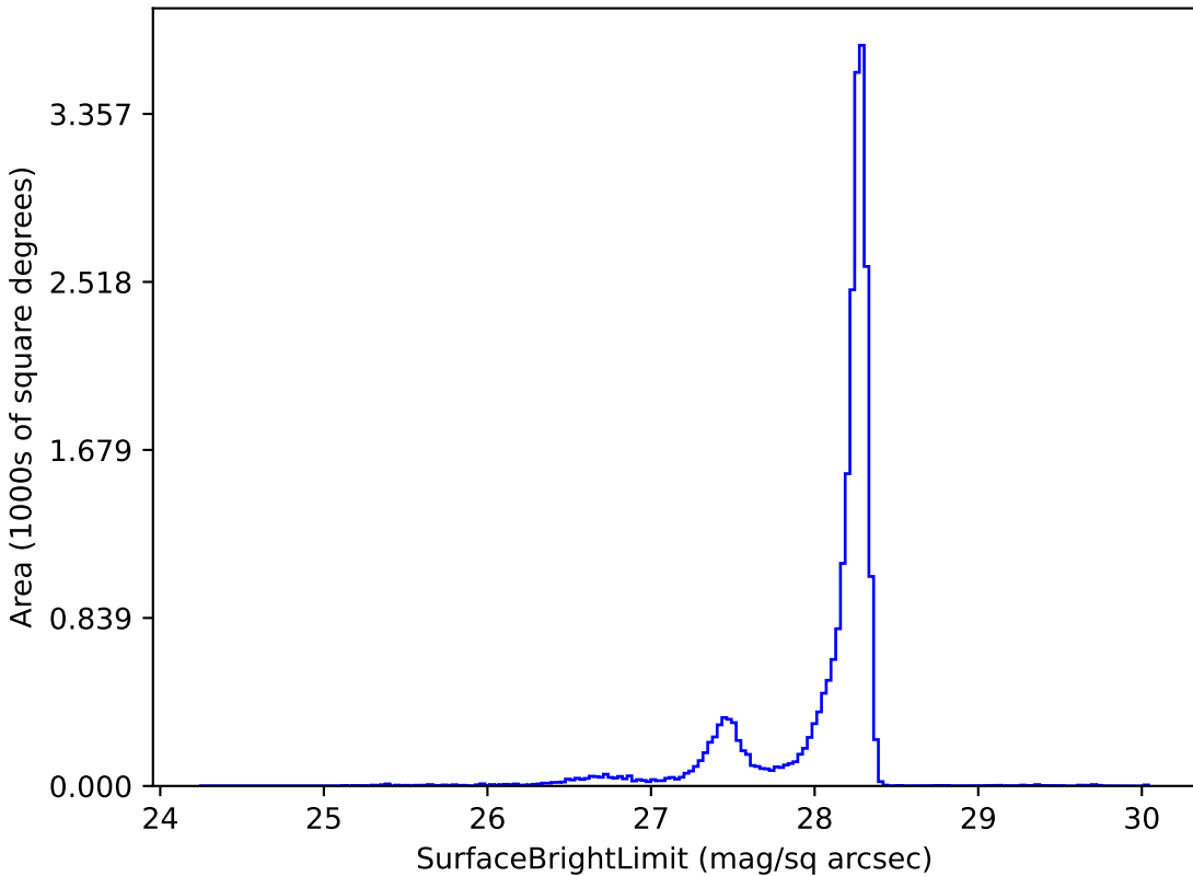
weather_cloudso36v3.4_10yrs y: SurfaceBrightLimit
