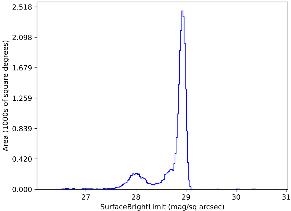
weather_cloudso36v3.4_10yrs u: SurfaceBrightLimit
