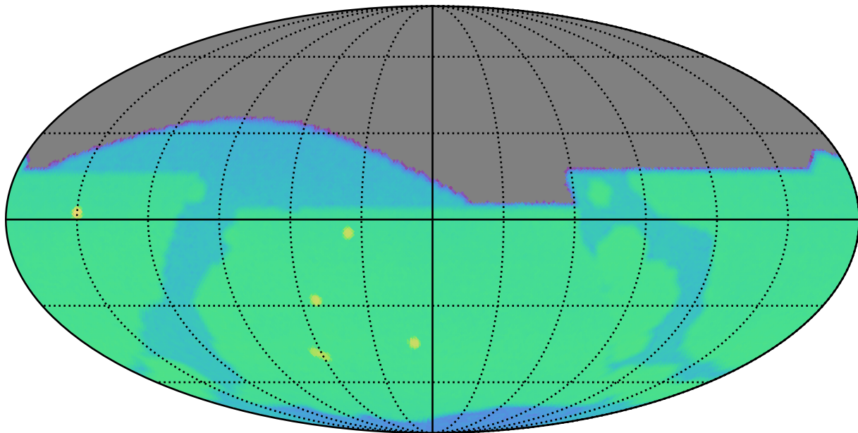
weather_cloudso36v3.4_10yrs r: SurfaceBrightLimit
