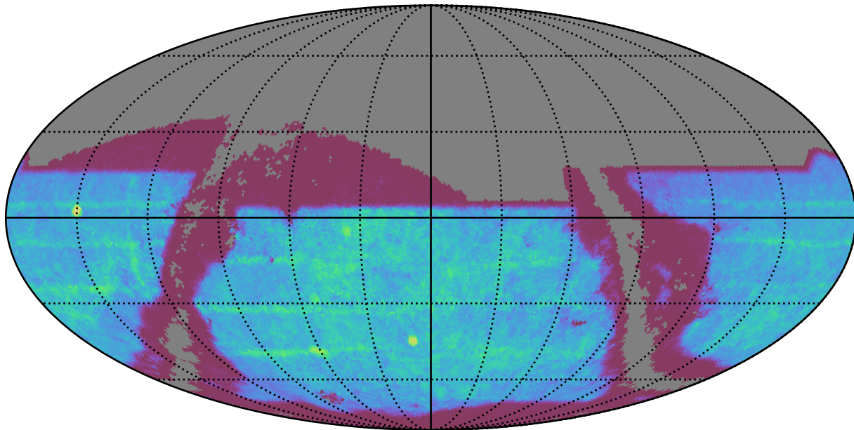
weather_cloudso36v3.4_10yrs : SNSLMetric
