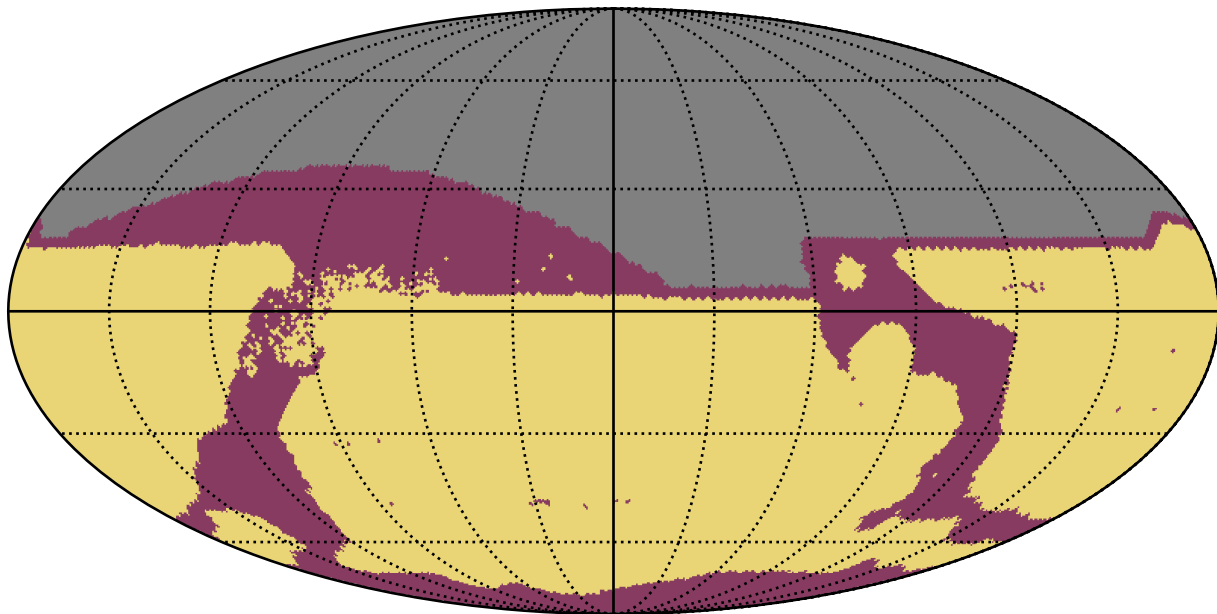
weather_cloudso36v3.4_10yrs : RapidRevisits
