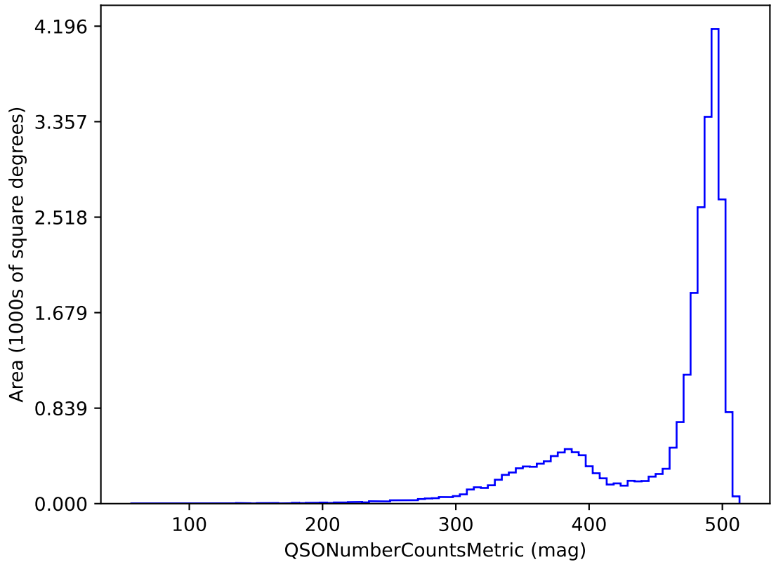
weather_cloudso36v3.4_10yrs z band and non-DD: QSONumberCountsMetric
