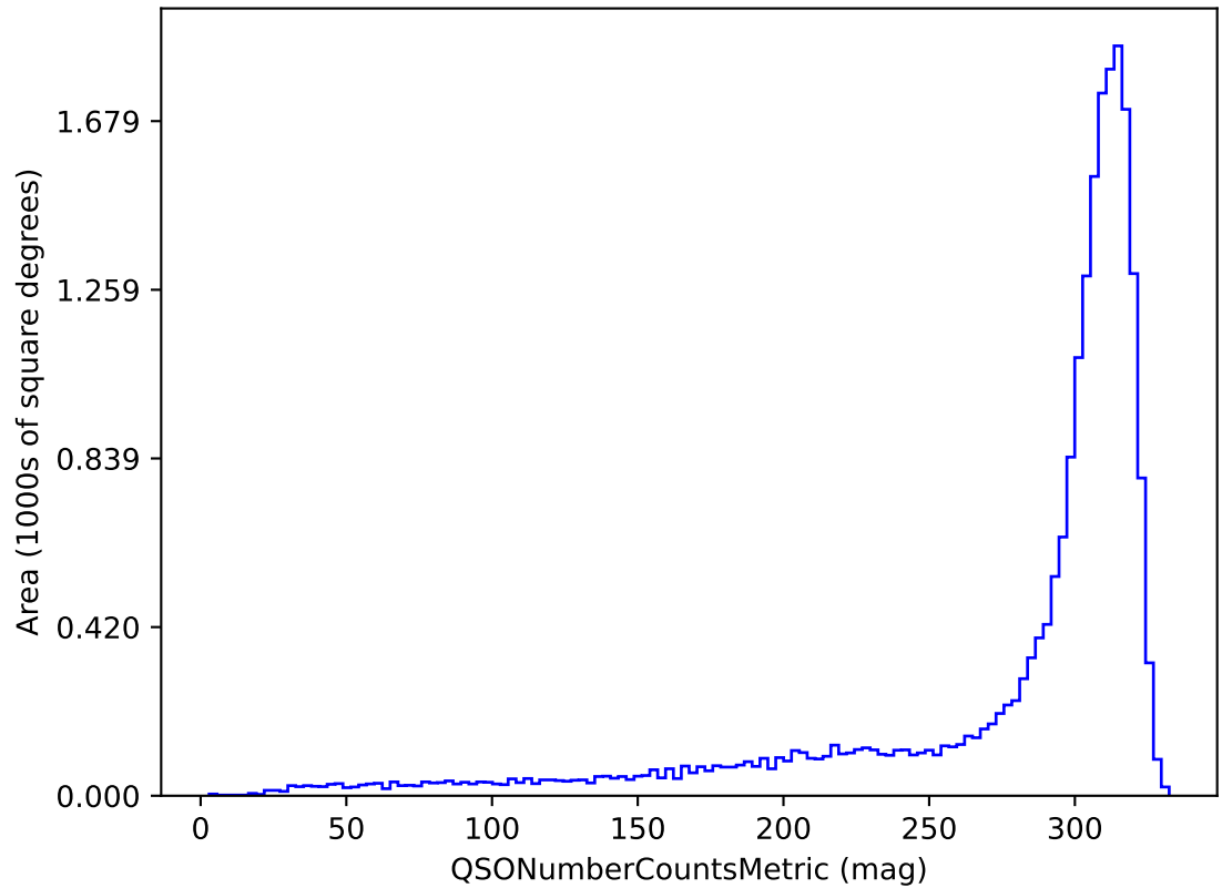
weather_cloudso36v3.4_10yrs u band and non-DD: QSONumberCountsMetric
