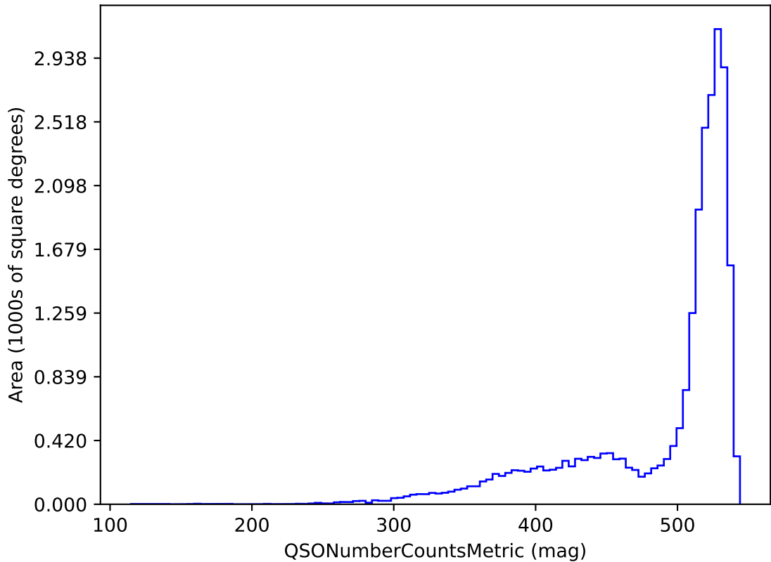
weather_cloudso36v3.4_10yrs r band and non-DD: QSONumberCountsMetric
