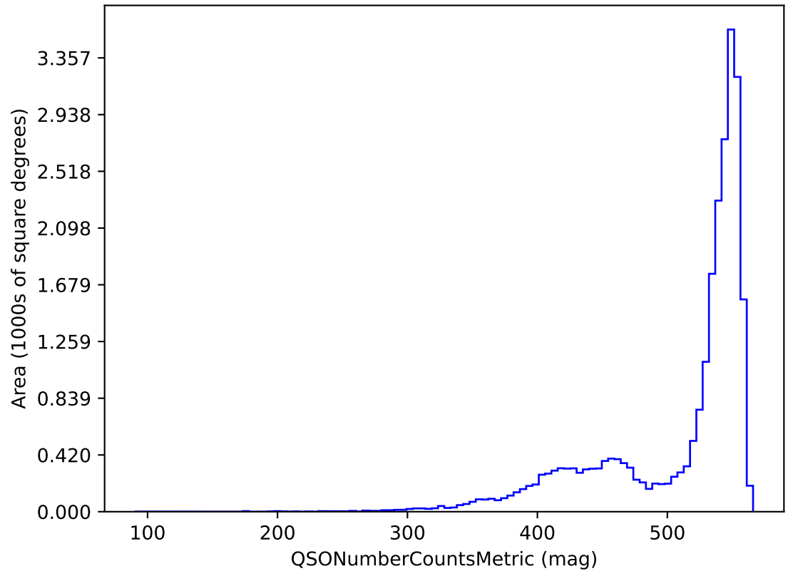
weather_cloudso36v3.4_10yrs i band and non-DD: QSONumberCountsMetric
