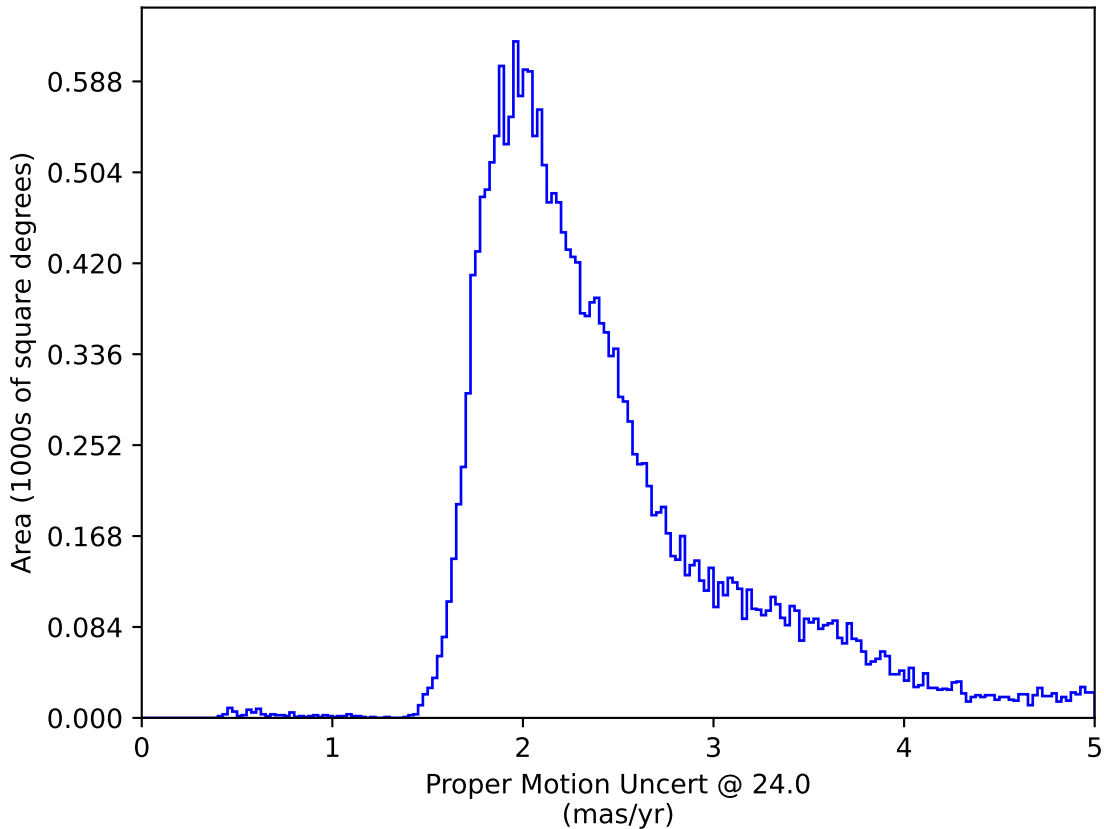
weather_cloudso36v3.4_10yrs : Proper Motion Uncert @ 24.0
